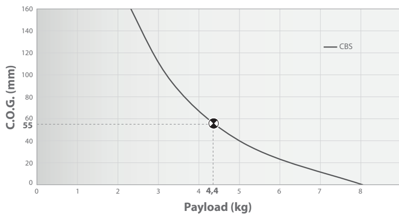
COUNTERBALANCE GRAPH MVH502XAH (21°C)
